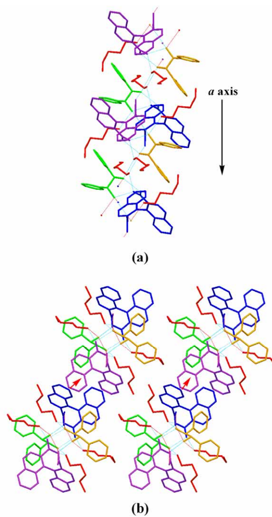
Fig. S1. Crystal structure of complex III . (a) Column structure is parallel to the a axis. (b) Packing structure observed along the a axis. Red arrows show naphthalene-naphthalene edge-to-face interactions.
