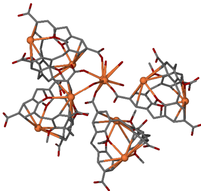
Figure S1. The additional Rb-carboxylate bonding found in 4·Rb.
