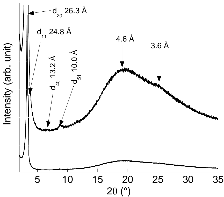
Fig. 2 X-Ray diffraction pattern of 3F at 220 °C
