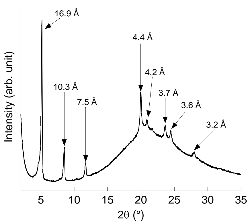
Fig. 1 X-Ray diffraction pattern of 2F6F at 140 °C
