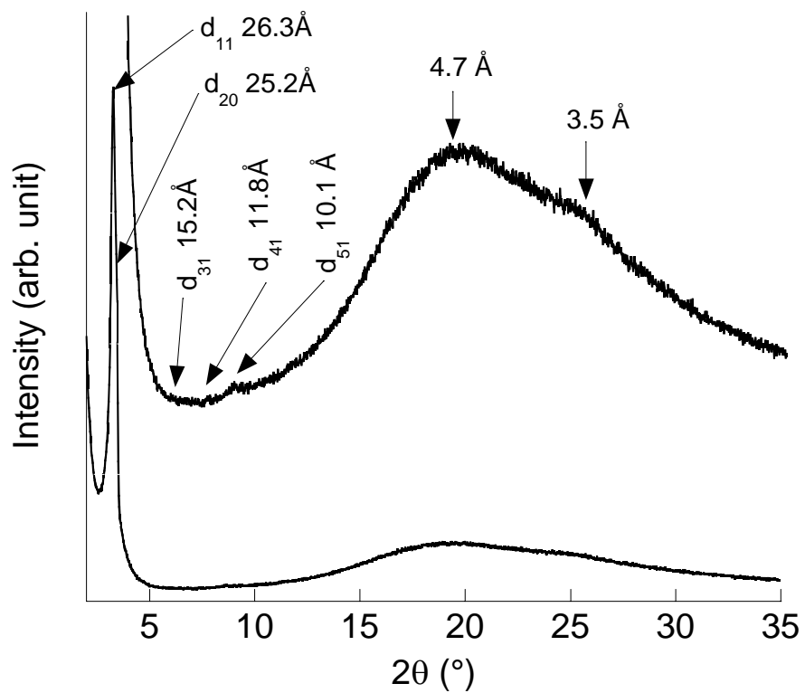
Fig.3 X-Ray diffraction pattern of 3F at 250 °C
