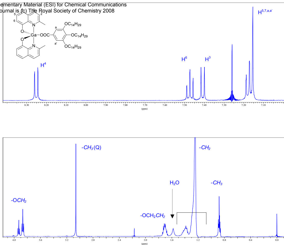
Figure S2. Proton numbering scheme and 1 H NMR spectrum of GaQL, in CDCl 3 .
