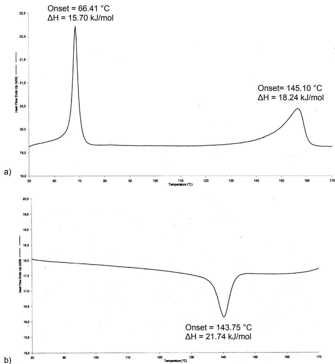
Figure S1. DSC thermograms for the complex GaQ 2 L : a) heating and b) cooling scan.
