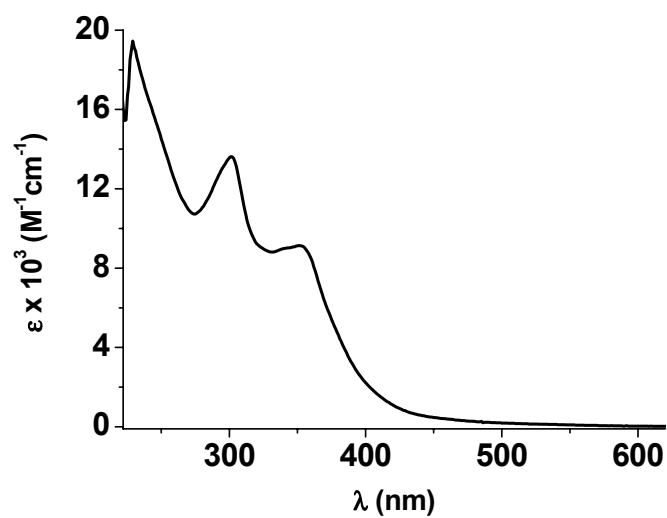
ESI S1 UV-vis spectrum of [Fe_2O(L)Cl_4] at rt in CH_2Cl_2 solutions.
