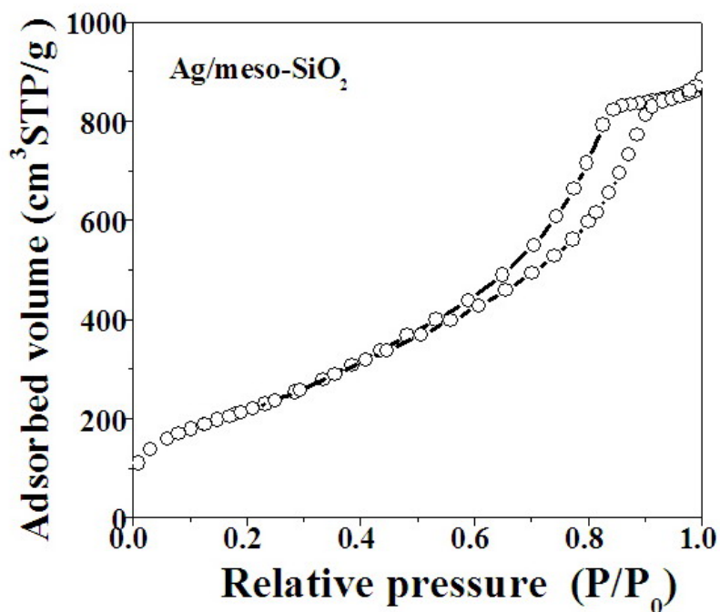
Figure S1 Nitrogen adsorption isotherm profile of Ag/meso-SiO 2 measured at 77 K
