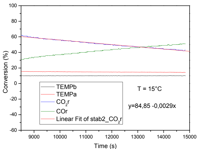
Figure S1. Deactivation plot for \text{Co}_3\text{O}_4 -40 catalyst
