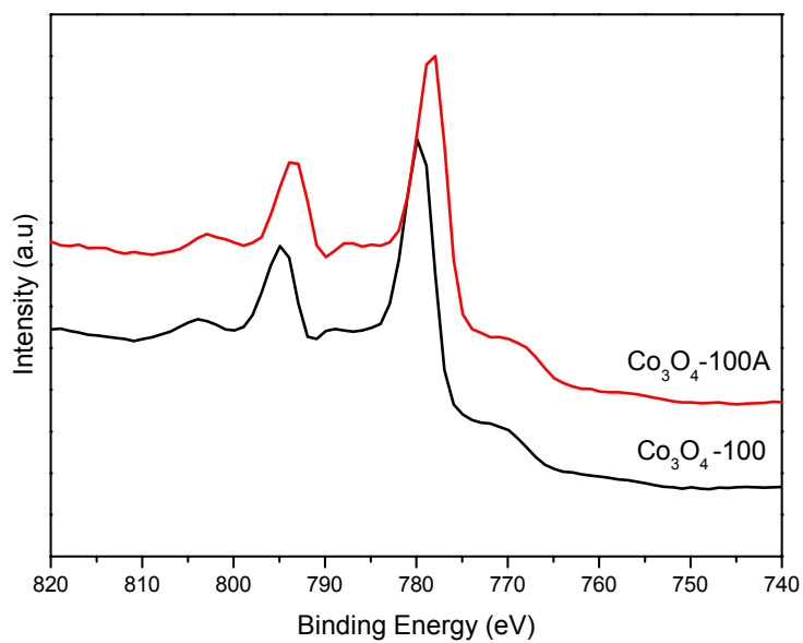
Figure S2. XPS spectrum for Co 3 O 4 -100 before and after catalytic test.
