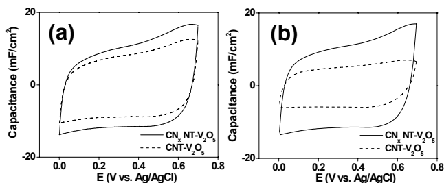
Figure S1 CV curves of V_2O_5 on N-doped and undoped CNTs performed (a) before and (b) after 1000-cycle tests. (Electrolyte: 1 20 M KCl and 1 M KHSO_4 )
