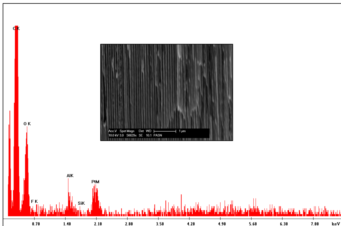
Figure 2. EDX spectra of the cross-section of membranes treated with PFPTES. (insets: SEM cross-section view of the membranes).
