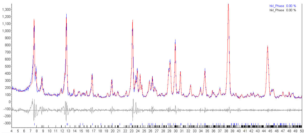
Fig. S2. LeBail fit of heteroepitaxially grown MFI (Bragg reflections are the black bars - down) on ETS-4 (Bragg reflections are the blue bars - up). The starting unit cell parameters and space group were taken from ref. [19] and [20].
