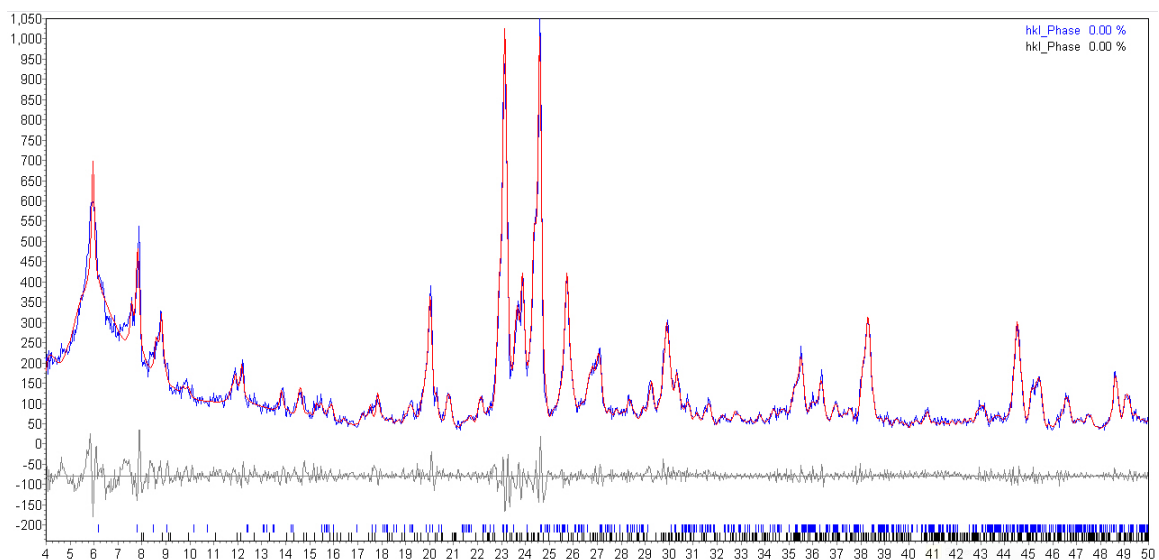
Fig. S1. LeBail fit of heteroepitaxially grown MFI (Bragg reflections are the black bars - down) on ETS-10 (Bragg reflections are the blue bars - up). The starting unit cell parameters and space group were taken from ref. [18] and [19].
