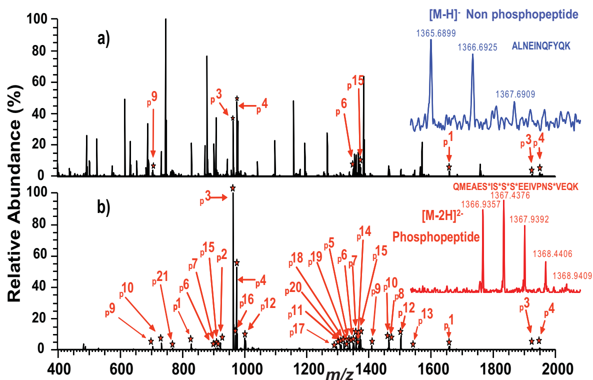
Fig. S3 ESI/FTMS spectra of peptide mixtures digested from \alpha -casein with trypsin (a) before and (b) after enrichment using mesoporous \text{ZrO}_2 . Phosphopeptides are labeled with numbers that are listed in Table S42. Insets show a singly charged non phosphopeptide in (a) and a doubly charged quintuply phosphorylated peptide, p14, in (b).
