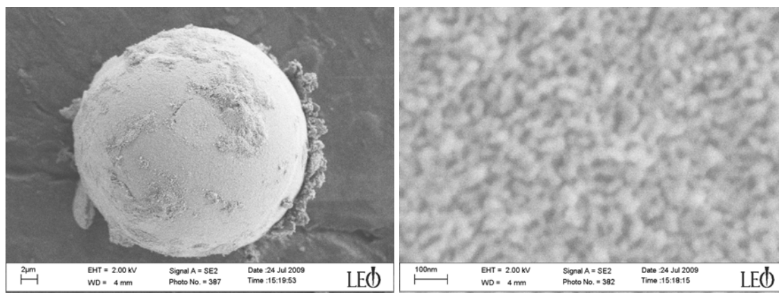
Fig. S4 Representative SEM images of the commercial phosphoenrichment materials based on \text{ZrO}_2 , which consist of microspheres of aggregates of \text{ZrO}_2 nanoparticles of about 20 nm diameter. This was the materials used for enrichment experiment shown in Fig. 2B.
