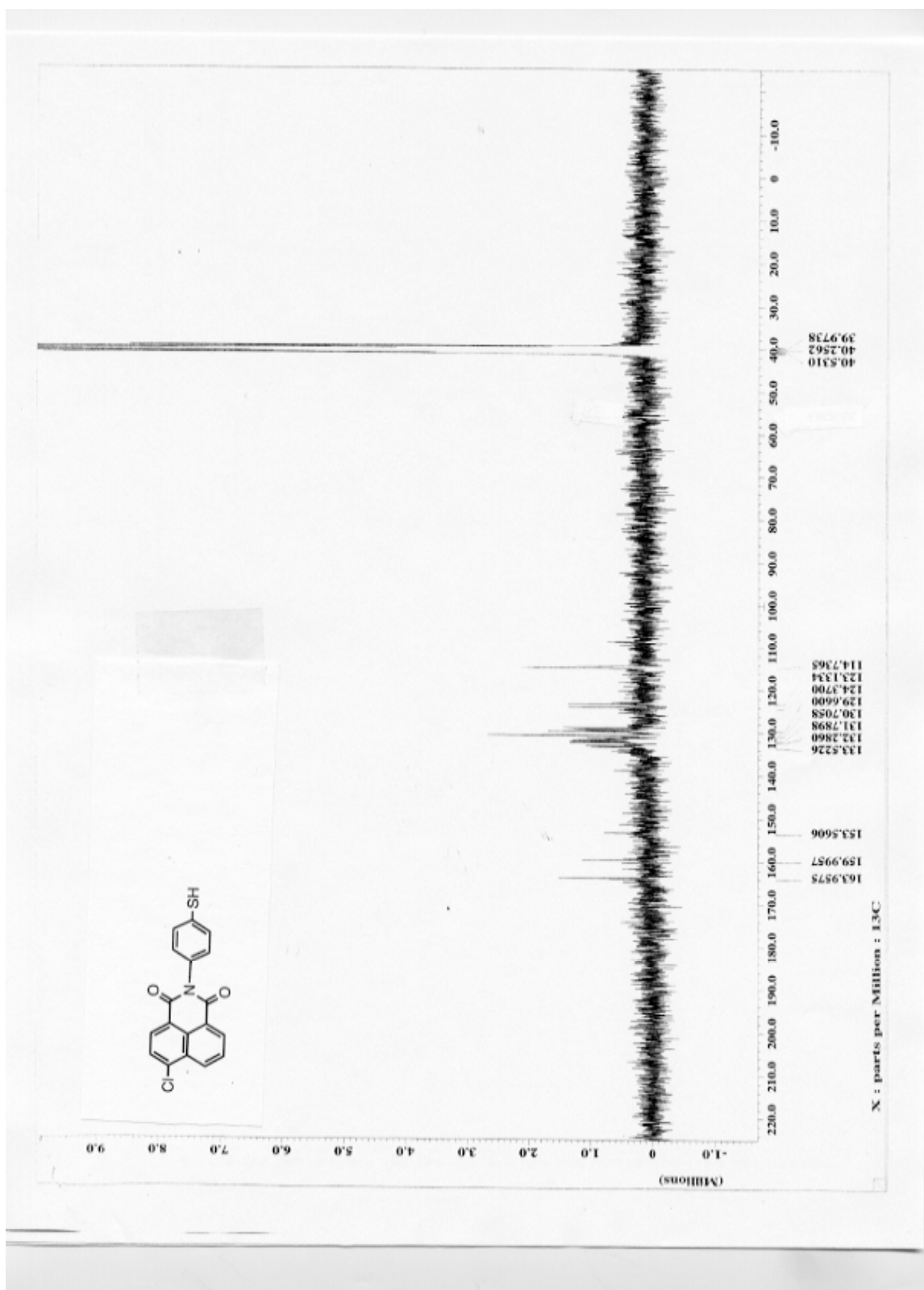
13 C NMR for 4-thiophenyl-1,8-NI (9)
