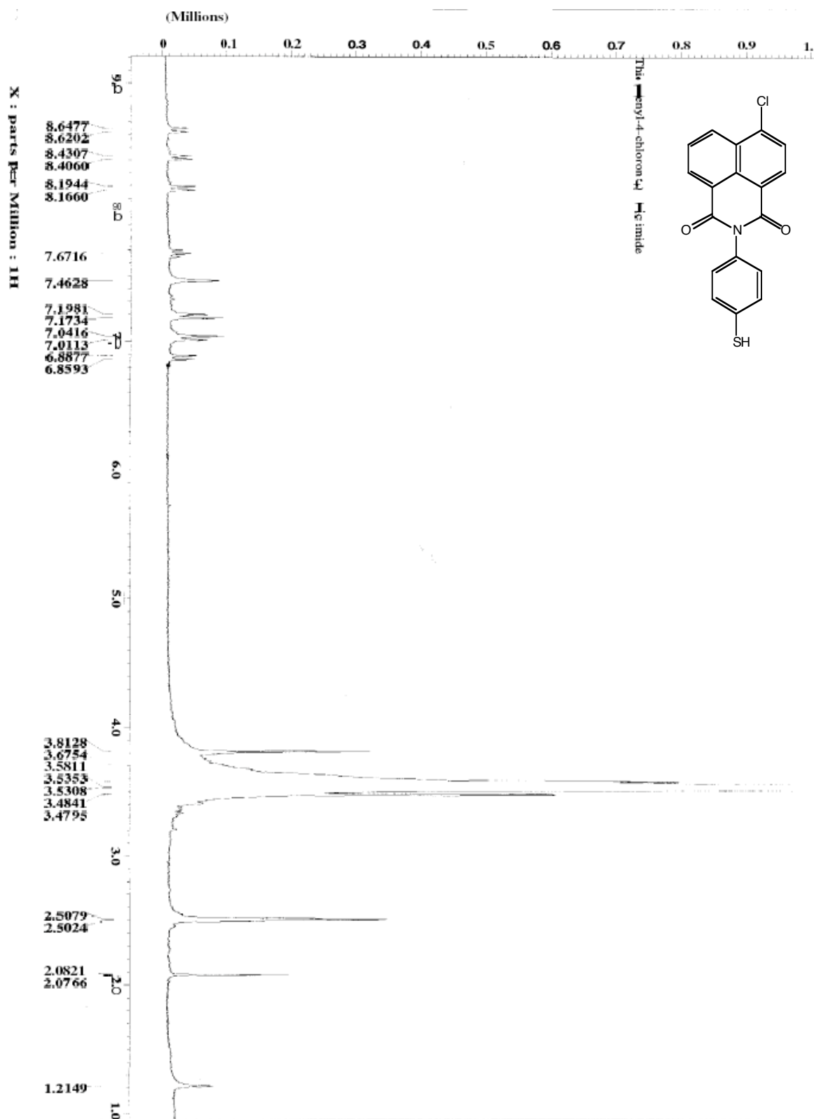
1 H NMR for 4-thiophenyl-1,8-NI (9)
