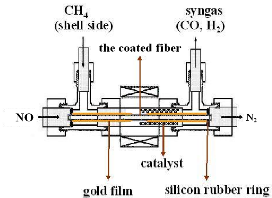
Figure S1 Schematic diagram of the membrane reactor used in this work
