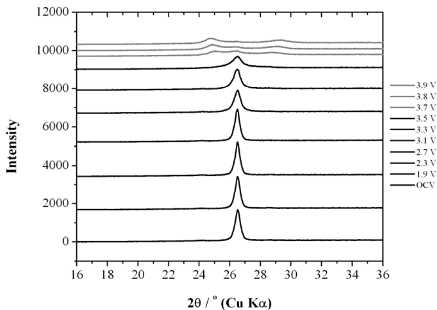
Fig. S1b in situ XRD patterns of the KS6 positive electrode in the capacitors using the electrolyte solutions of 1.5M SBPBF 6 dissolved in EC.
