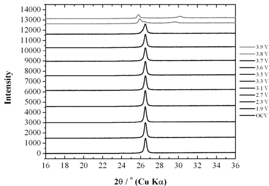
Fig. S1a in situ XRD patterns of the KS6 positive electrode in the capacitors using the electrolyte solutions of 1.5M SBPBF 6 dissolved in PC.
