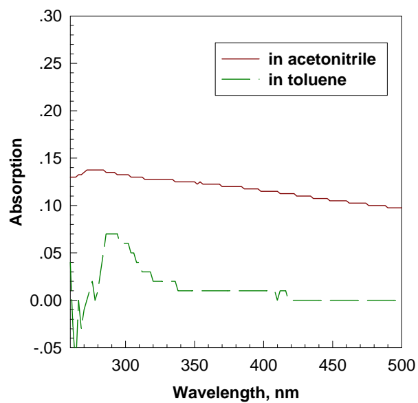
Figure S2. Absorption of PMDI in solvents at saturated concentration.
