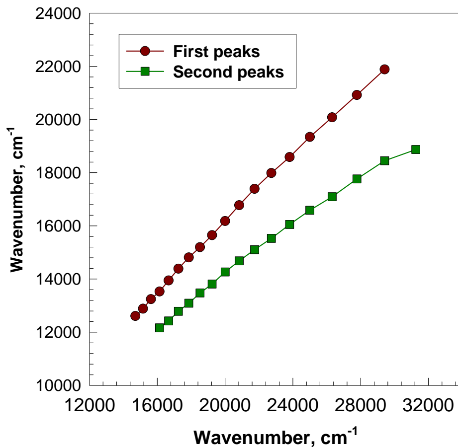
Figure S1. Photoluminescence peaks of PMDI nanowires (in the unit of wavenumber).
