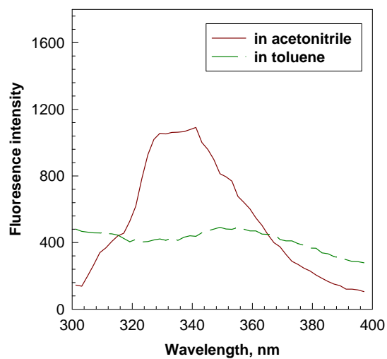
Figure S3. Fluorescence of PMDI in solvents at saturated concentration.
