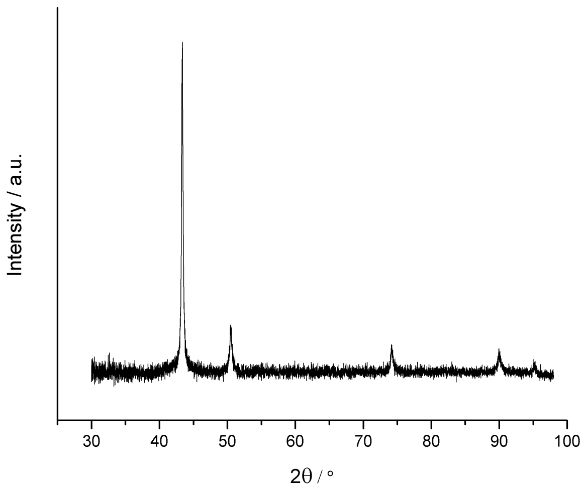
Fig. S1 XRD reflection pattern of a sample coated with copper before applying the silver nitrate containing solution. Only metallic copper was detected; the absence of any oxides was confirmed.
