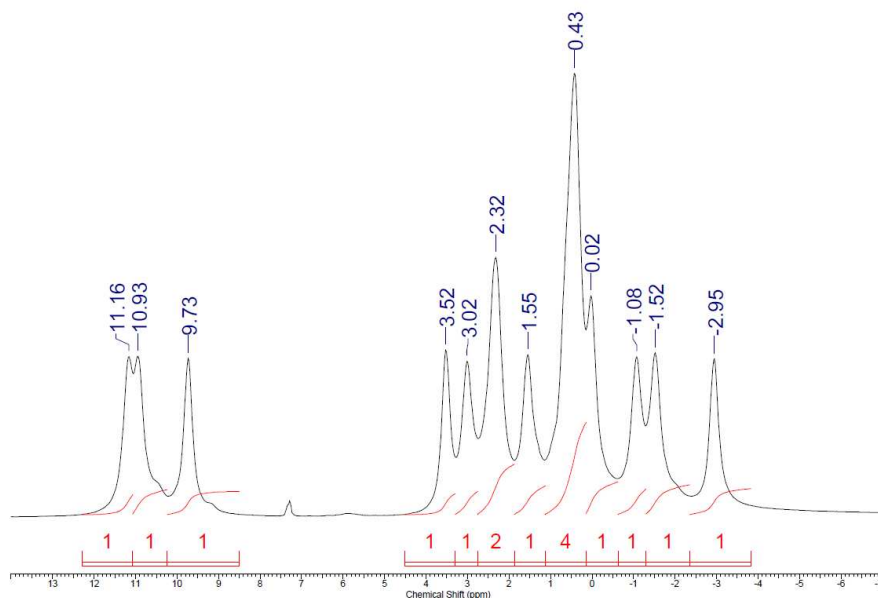
Figure S1. ^1\text{H} -NMR spectrum of 1 [(\text{H}_3\text{N}^{\text{Pr}})\text{Cr}_7\text{CoF}_8(\text{tBuCO}_2)_{16}] at 300MHz in \text{CDCl}_3 (Pivalate region)
