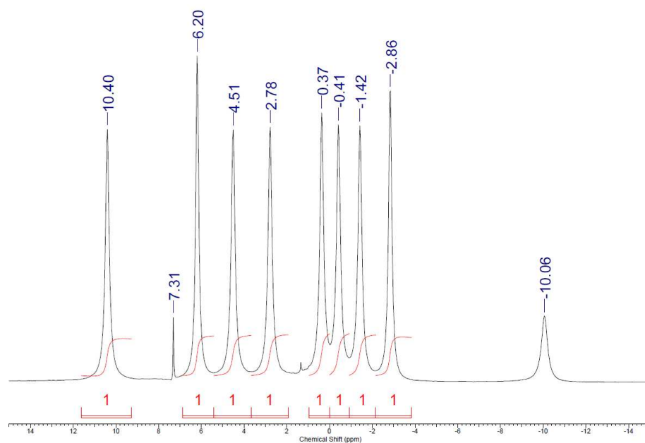
Figure S2. ^1\text{H} -NMR spectrum of 2 [\text{Cs} \subset \text{Cr}_7\text{MF}_8(\text{tBuCO}_2)_{16}] at 300MHz in \text{CDCl}_3 (Pivalate region)
