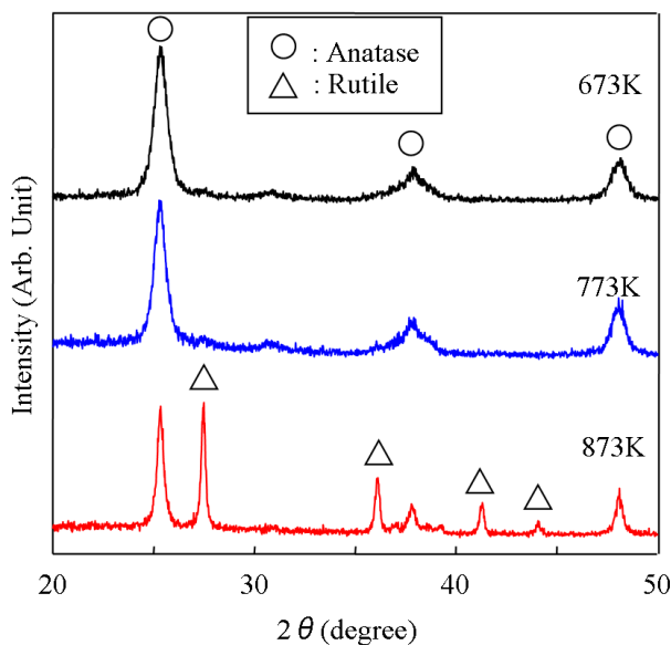
Figure S1. X-ray diffraction patterns of TiO 2 films that are prepared at different thermal treatment temperatures
