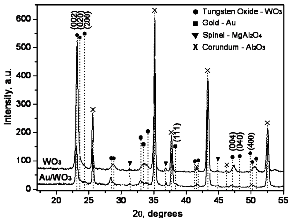
Fig. 1 XRD pattern of NP Au/WO 3 NN deposited via AACVD compared with non-functionalised WO 3 NN. 19
