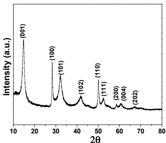
Fig. S1 X-ray diffraction (XRD) pattern of the as-synthesized SnS 2 nanosheets.
