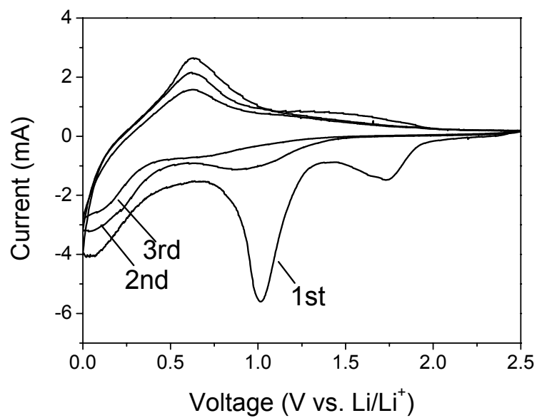
Fig. S3 Cyclic voltammogram of the SnS 2 electrode.
