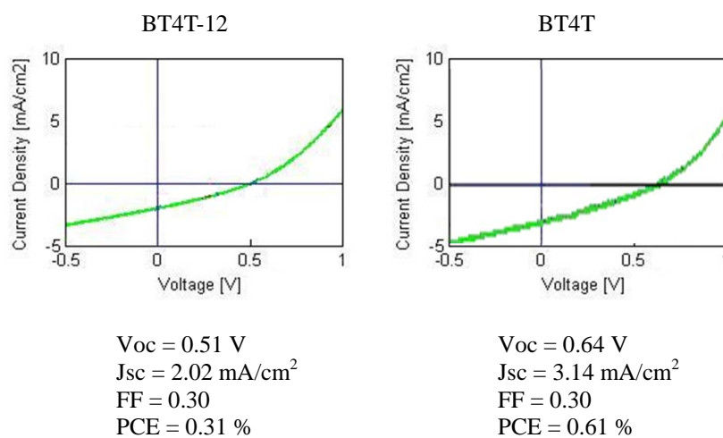
Figure S1. J-V curves of oligomers
