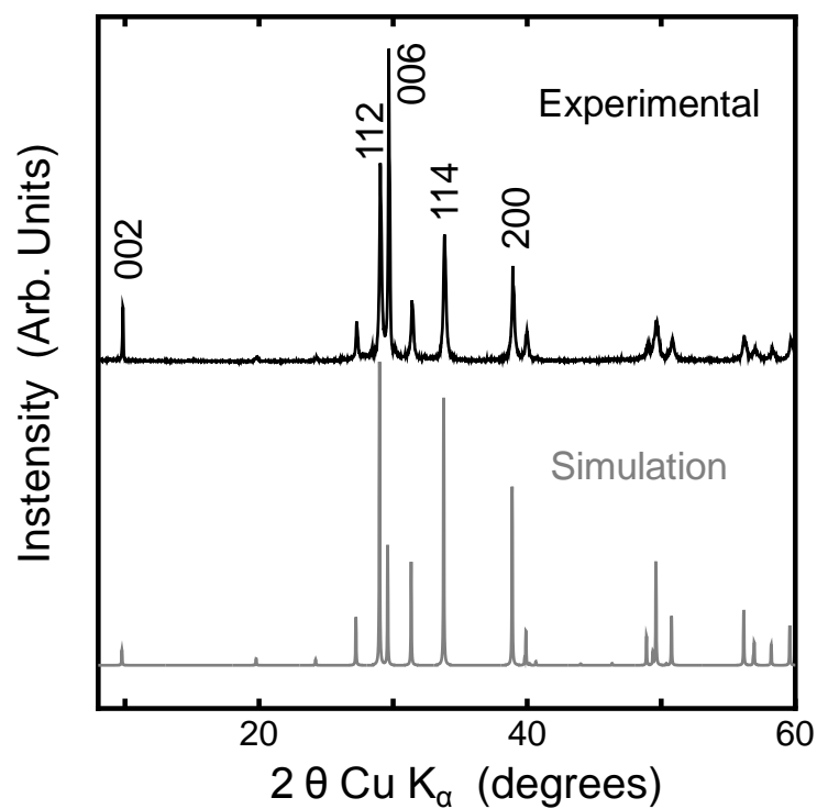
Figure S1. Powder XRD pattern of the \text{La}_2\text{Sb} sample, together with simulation pattern based on the structural data obtained from single crystal structure analysis. 11 Strong influence due to preferred orientation is seen.
