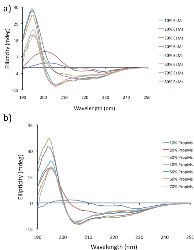
Figure S2: Far CD spectrum of modified beta peptide in a) ethylammonium mesylate b) propylammonium mesylate
