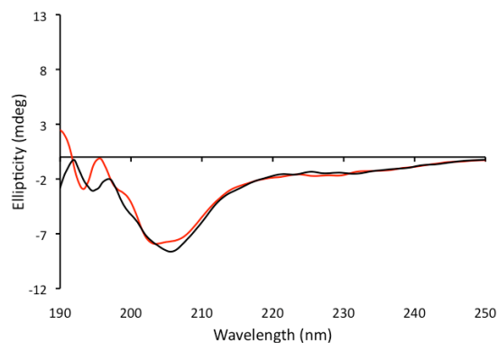
Figure S1: Far CD spectrum of ABeta 1-40 in aqueous pIL solution, at TeaMs concentrations of 90wt% (red), 100wt% (black).
