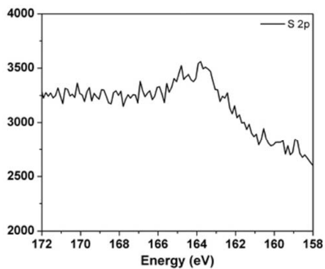
Figure S3, XPS spectrum of PAVS sphere
