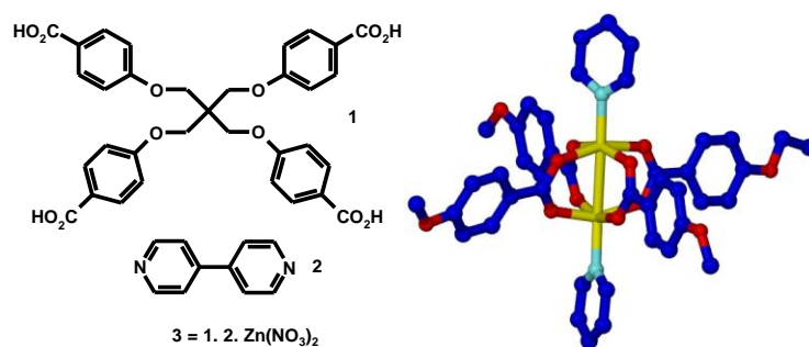
Scheme 1. Precursors used in the synthesis of TetZB and corresponding SBU unit.
