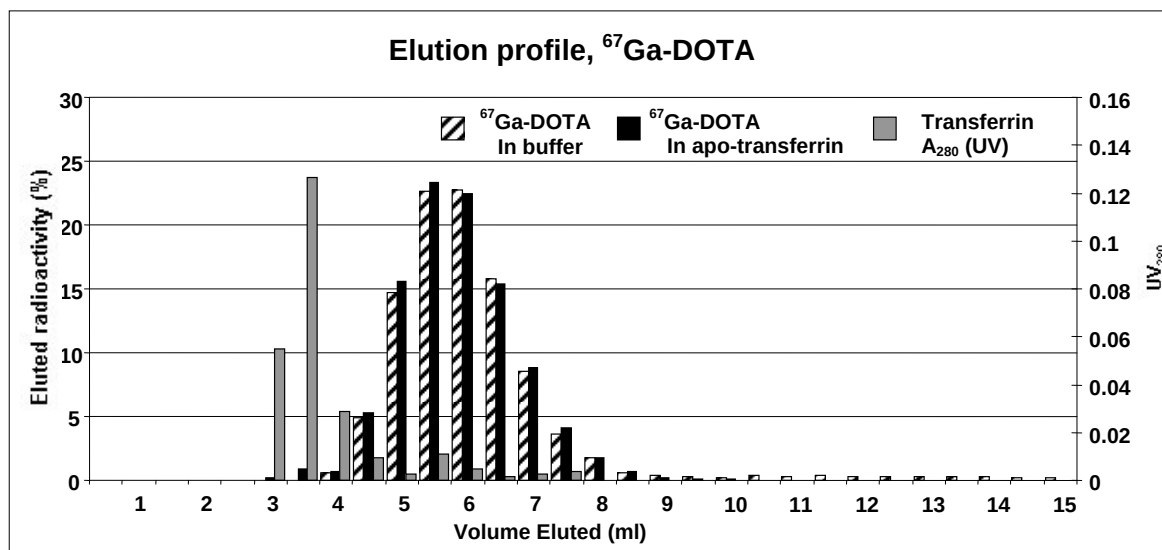
Figure S9. Gel filtration elution profile of ^{67}\text{Ga} -DOTA complex after 4 hours incubation in apo-transferrin solution; 100 \mu\text{M} DOTA radiolabelling concentration.
