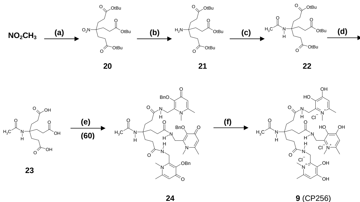
Scheme S2. Synthesis of tripodal chelator CP256 ( 9 ). Materials and methods: (a) Triton B, Tert-butyl acrylate, DME, 70°C; (b) T-1 Raney Ni, H 2 , 25°C, EtOH; (c) CH 3 COCl, Et 3 N, CH 2 Cl 2 , 0-25°C, (d) HCOOH; (e) 19 , DCCl, HoBt, DMF 25°C; (f) Pd/C, H 2 , HCl, CH 3 OH, 25°C.
