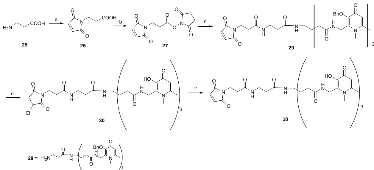
Scheme S3: Synthesis of maleimide linked hexadentate chelator 10 . a) maleic anhydride/DMF; b) DCC/NHS/DMF; c) 28 /DMF; d) BCl 3 /DCM; e) Et 3 N/DCM.
