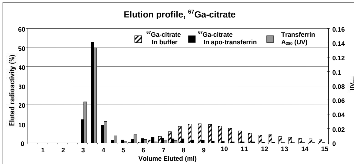
Figure S8. Gel filtration on PD10 column. (A) Elution profile of ^{67}\text{Ga} -citrate complex after incubation with apo-transferrin after 4 hours incubation. The UV elution profile of apo-transferrin is also shown.
