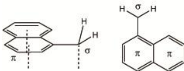
Scheme S1 : Schematic representations of the \pi + \sigma -bonded surface species formed by partially dehydrogenated methylnaphthalene on Pt(111) at room temperature.
