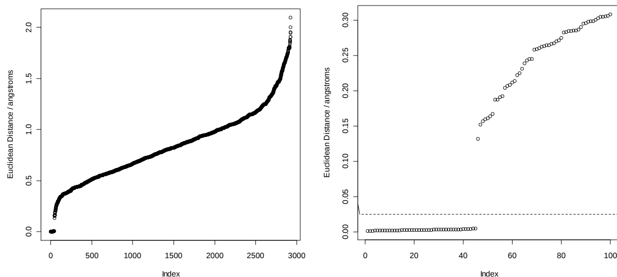
Figure 5: Plot of inter-structure Euclidean distances of minimum basis from all Rhodobacter bacteriopheophytin cofactors.
