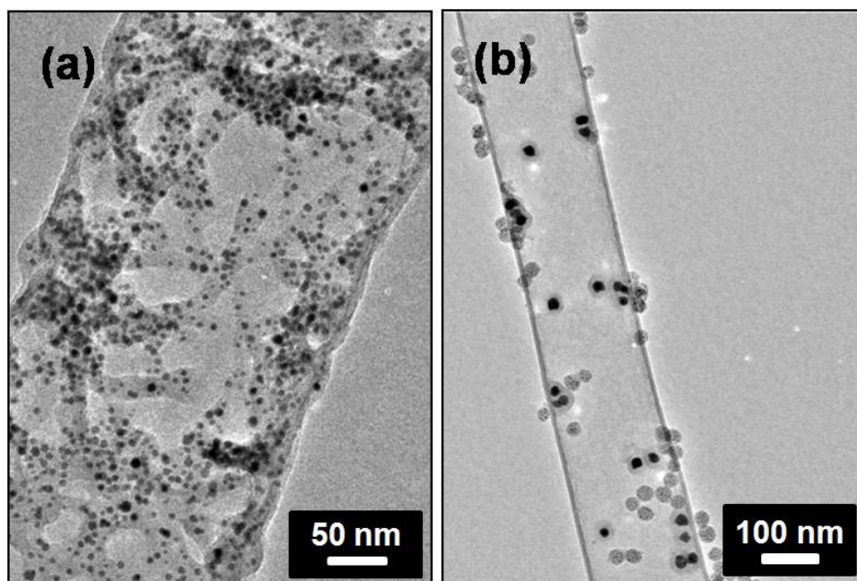
Figure S2. TEM images of hCNTs-1 containing Au NPs (a) and hCNTs-2 containing Pt NPs (b).
