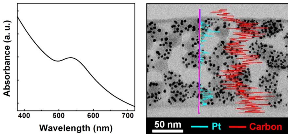
Figure S3. UV-visible absorption spectrum of hCNTs-2 containing Au NPs (left). Magnified TEM image and EDX line-scan profiles of a hCNT-1 containing Pt NPs (right).
