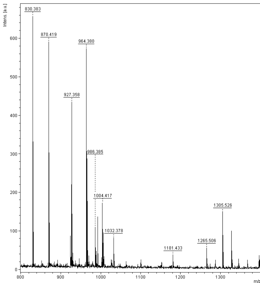
Fig. 11 a. Resin bound library constructed from A1, A2, C1, C2 in solution and resin bound B1 and B2 (10:10:10:10:1:1) after 2 weeks of equilibration in the presence of aniline at pH 7.4
