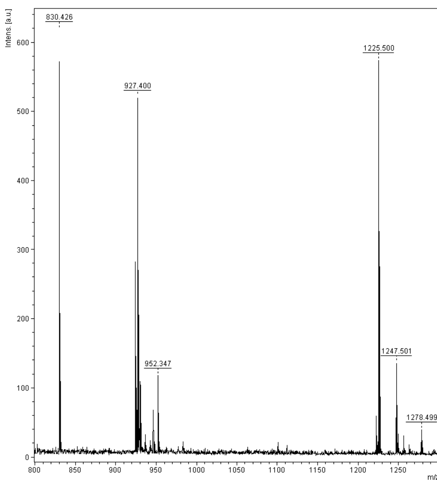
Fig. 9. Resin bound library constructed from A1 and C1 in solution and resin bound B1 (10:1:10 ratio) after 6 days of equilibration in the presence of aniline at pH 7.4
