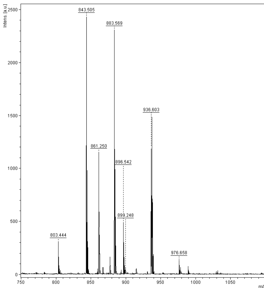
Fig. 3. Solution phase library constructed from A1, A2, B1 and B2 after 3 days of equilibration in the presence of thiopropanol at pH 7.4
