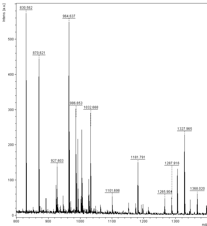
Fig. 10 a. Resin bound library constructed from A1, A2, C1, C2 in solution and resin bound B1 and B2 (10:10:10:10:1:1 ratio) after 1 week of equilibration in the presence of aniline at pH 7.4
