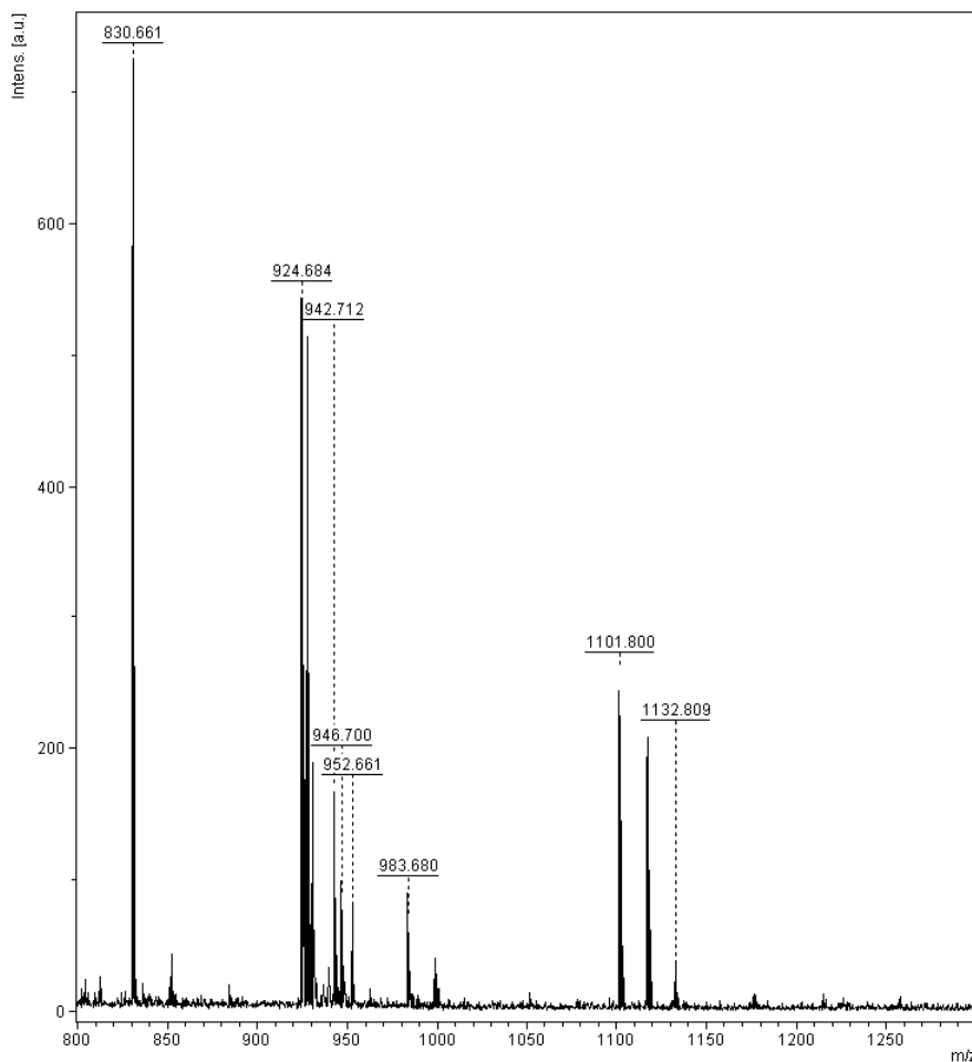
Fig. 8. Resin bound library constructed from A1 and C1 in solution and resin bound B1 (1:1:1 ratio) after 6 days of equilibration in the presence of thiopropanol at pH 7.4
