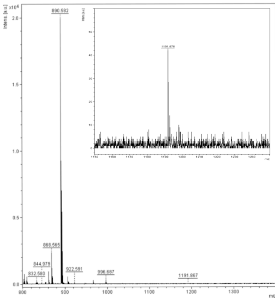
Fig. 4. Solution phase library constructed from A1, B1, and C1 after 3 days of equilibration in the presence of aniline and thiopropanol at pH 7.4
