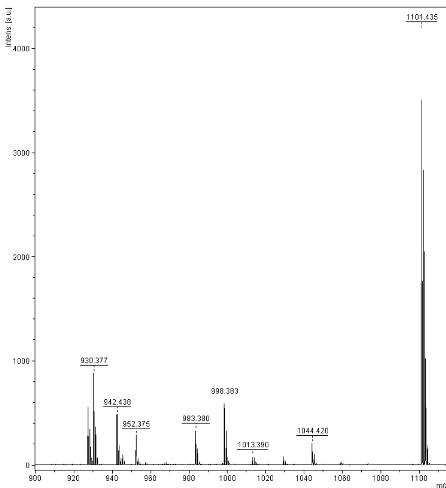
Fig. 7. Resin bound library constructed from A1 in solution and resin bound B1 after 6 days of equilibration in the presence of thiopropanol at pH 7.4
