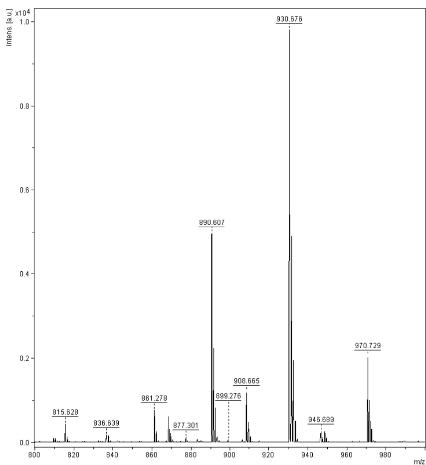
Fig. 2. Solution phase library constructed from B1, B2, C1, and C2 after 3 days of equilibration in the presence of aniline at pH 7.4
