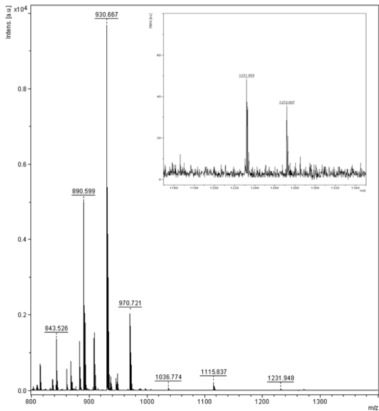
Fig. 5a. Solution phase library constructed from A1, A2, B1, B2, C1, and C2 (1:1:1:1:1:1 ratio) after 3 days of equilibration in the presence of aniline and thiopropanol at pH 7.4
