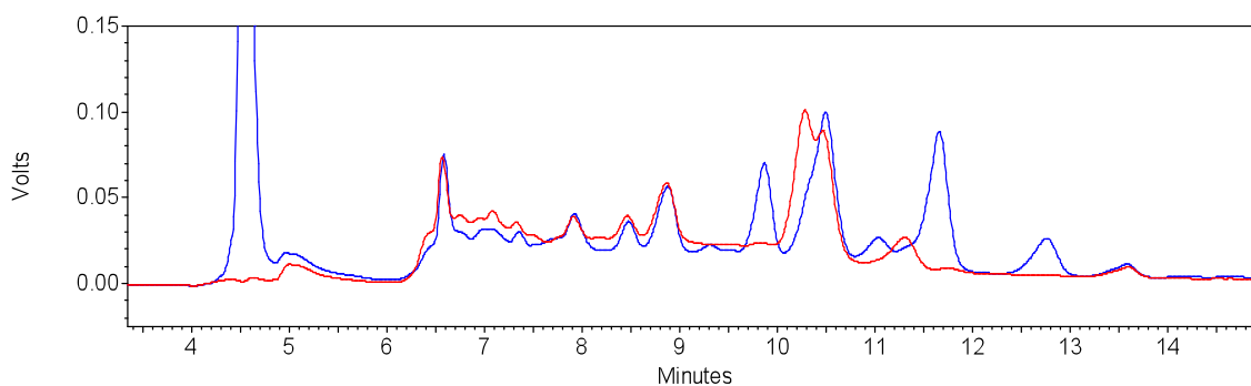
Fig. 1. Solution phase library constructed from B1, B2, C1, and C2 after 3 days of equilibration with aniline (blue trace) or without aniline (red trace) in ammonium acetate buffer (pH 7.4).
