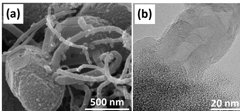
Fig. S2 High magnification (a) SEM and (b) TEM images of OMC-CNT nanocomposites.
