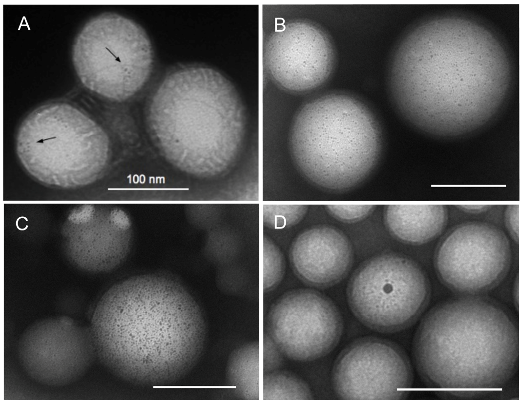
Figure 1. Zoomed out TEM images of lipid-PLGA nanoparticles with (A) AuNCs x1, (B) AuNCs x2, (C) AuNCs x3, (D) QDs x1. All scale bars are 100 nm.
