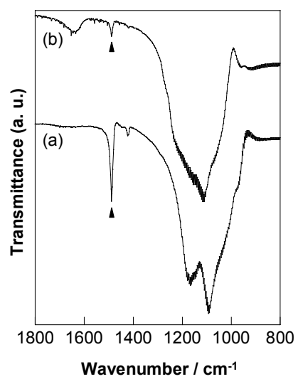
Fig. S2 FT-IR spectra of (a) HUS-1 and (b) DMS-HUS.
