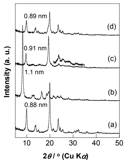
Fig. S1 XRD patterns of (a) HUS-1, DMS-HUS (b) before and (c) after washing, and (d) DMS-TMA-HUS.
