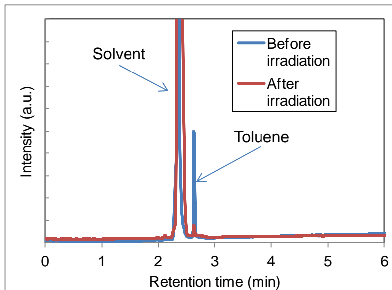
Fig.S2 HPLC charts for an aqueous toluene solution (1 mM) before and after irradiation of sunlight for 3 hours.
