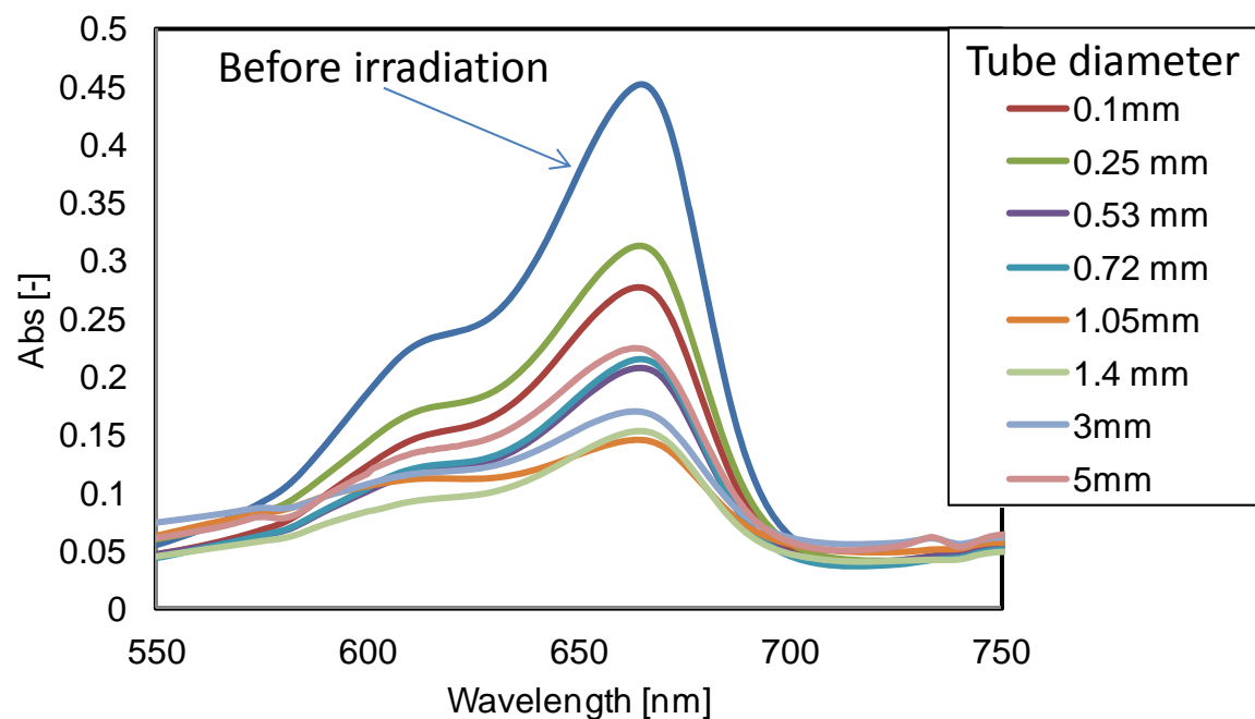
Fig.S1 The dependence of the inner diameter of photocatalytic microreactors on the absorption spectra of methylene blue solutions (10 \mu\text{M} ) after 1.5 hours irradiation of sunlight.
