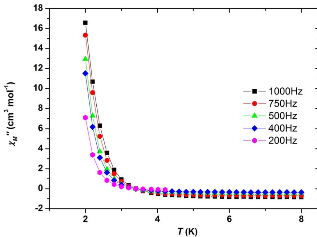
Figure S2. Plot of the out-of-phase ( \chi_M'' ) ac susceptibility versus temperature for 1 at the indicated frequencies.
