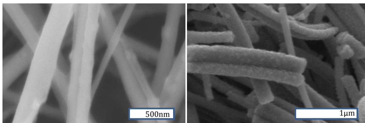
Figure S1. SEM micrographs illustrating the range of fiber sizes we are able to synthesize. The longitudinal contrast clearly indicates the biphasic nature of these fibers.
