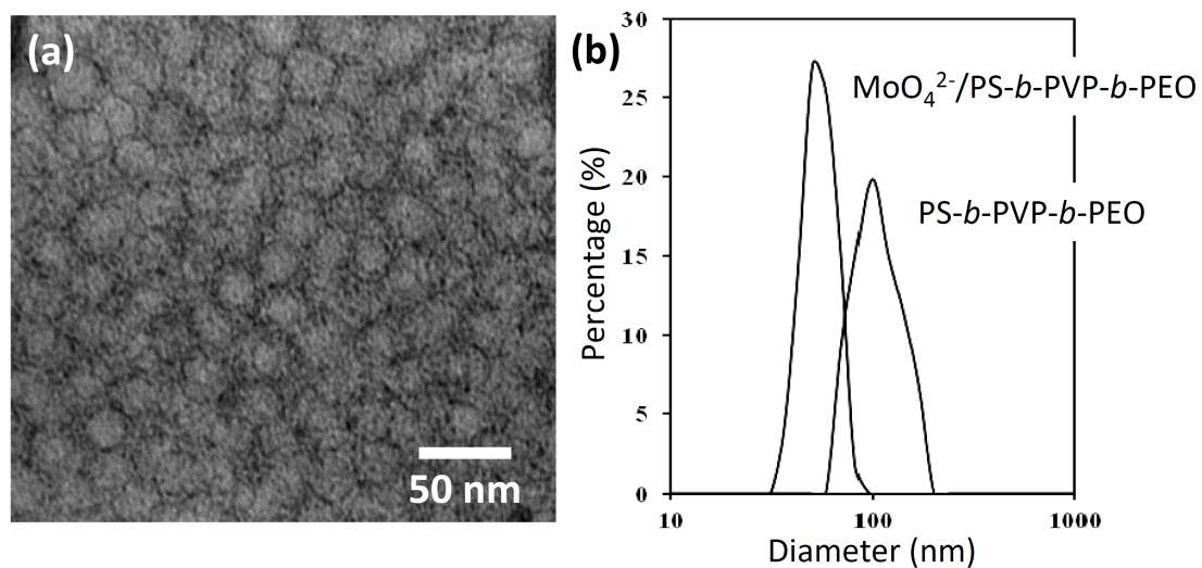
Figure S1 (a) TEM image of PS- b -PVP- b -PEO spherical micelles after staining with phosphotungstic acid. (b) Intensity-weighted contin plots for PS- b -PVP- b -PEO spherical micelles before and after addition of \text{MoO}_4^{2-} species.
