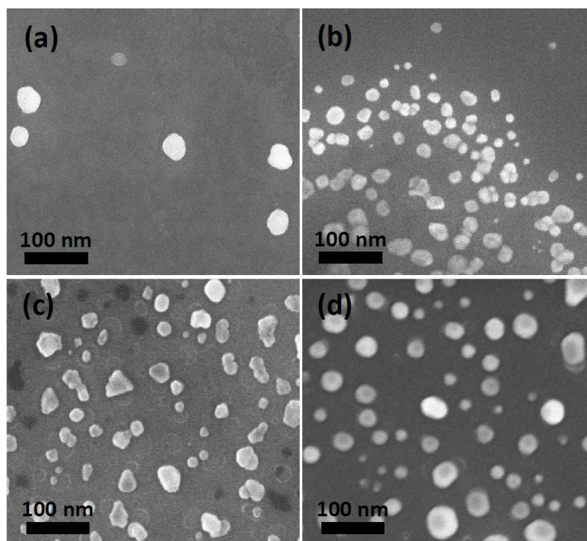
Figure S3 SEM image of samples prepared with PS- b -PVP diblock copolymer. Various annealing temperatures are applied ((a) 100 °C, (b) 200 °C, (c) 300 °C, and (d) 400°C).
