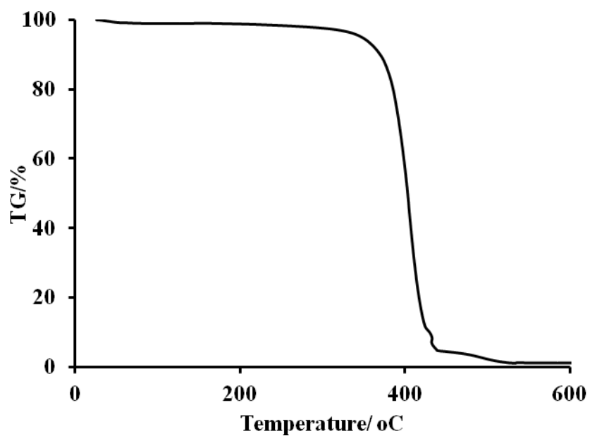
Figure S2 Thermogravimetric analysis of PS- b -PVP- b -PEO triblock copolymer.
