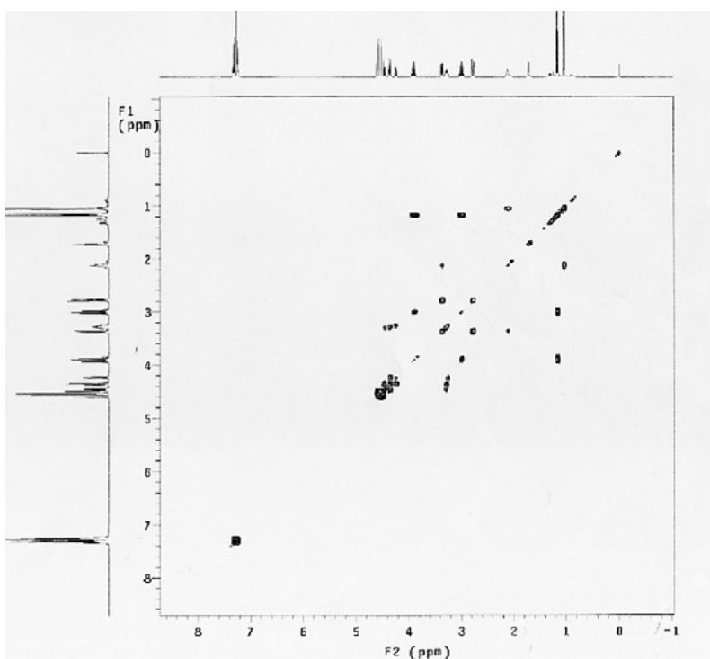
H-H COSY Spectrum
