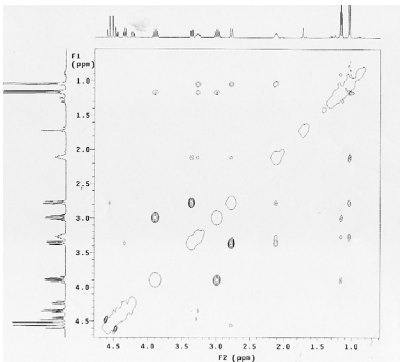
H-H NOESY Spectrum
