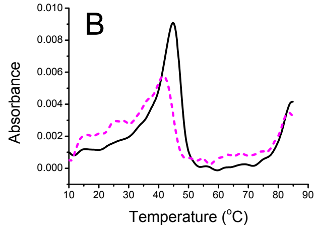
Thermal denaturation of Set 5 hp triplexes.
