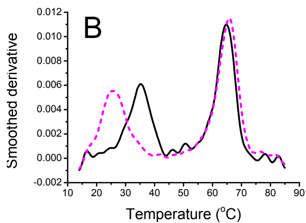
Thermal denaturation of Set 4 triplexes.
