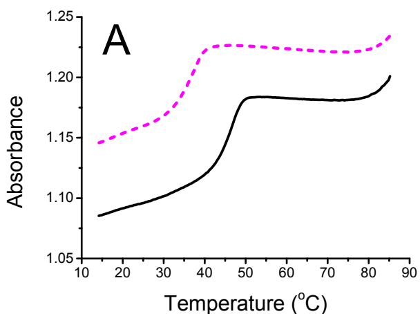
Thermal denaturation of Set 3 hp triplexes.
