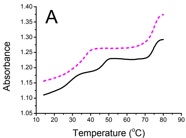
Thermal denaturation of Set 3 triplexes.
