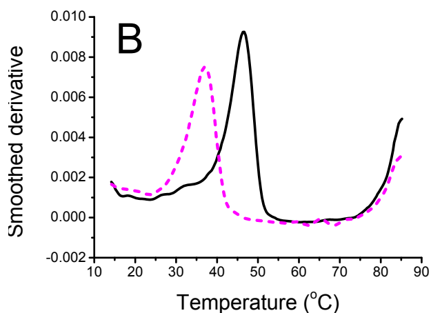
Thermal denaturation of Set 3 hp triplexes.
