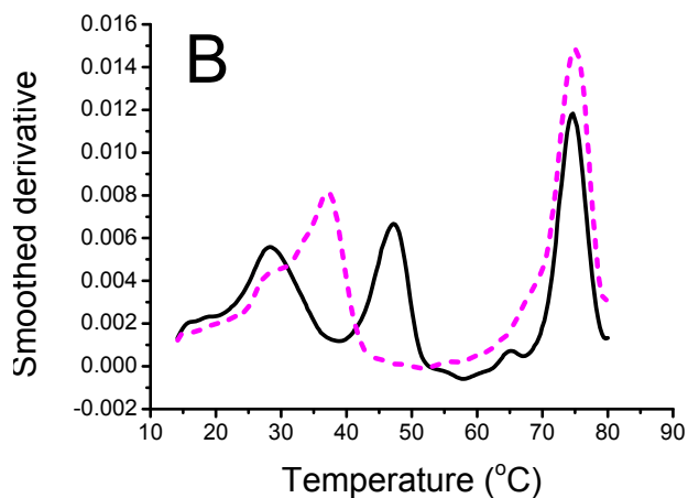
Thermal denaturation of Set 3 triplexes.
