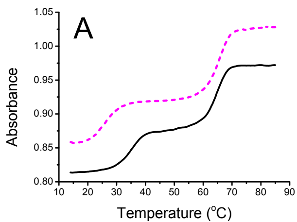
Thermal denaturation of Set 4 triplexes.
