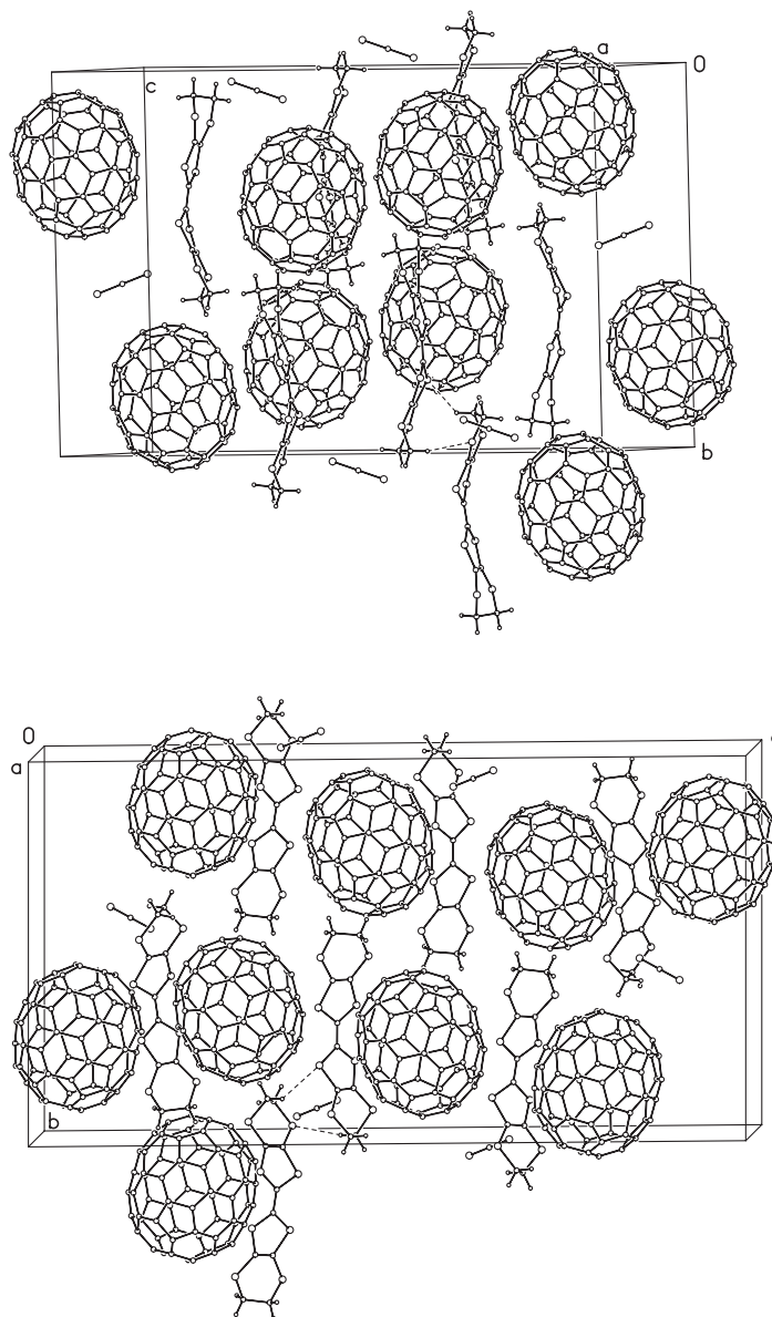
Figure S2. 2C_{70} \cdot 2ET \cdot CS_2 packing diagrams
