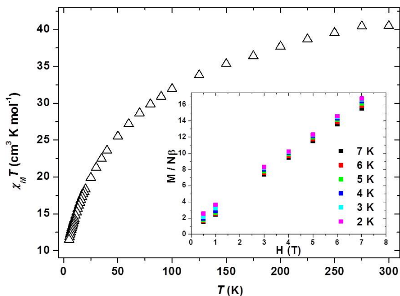
Figure S2. Plot of the \chi_M T product versus T for 1 in an applied field of 0.1 T. The inset shows magnetisation versus field data in the T = 2-7 K and H = 0.5 - 7.0 T temperature and field ranges.
