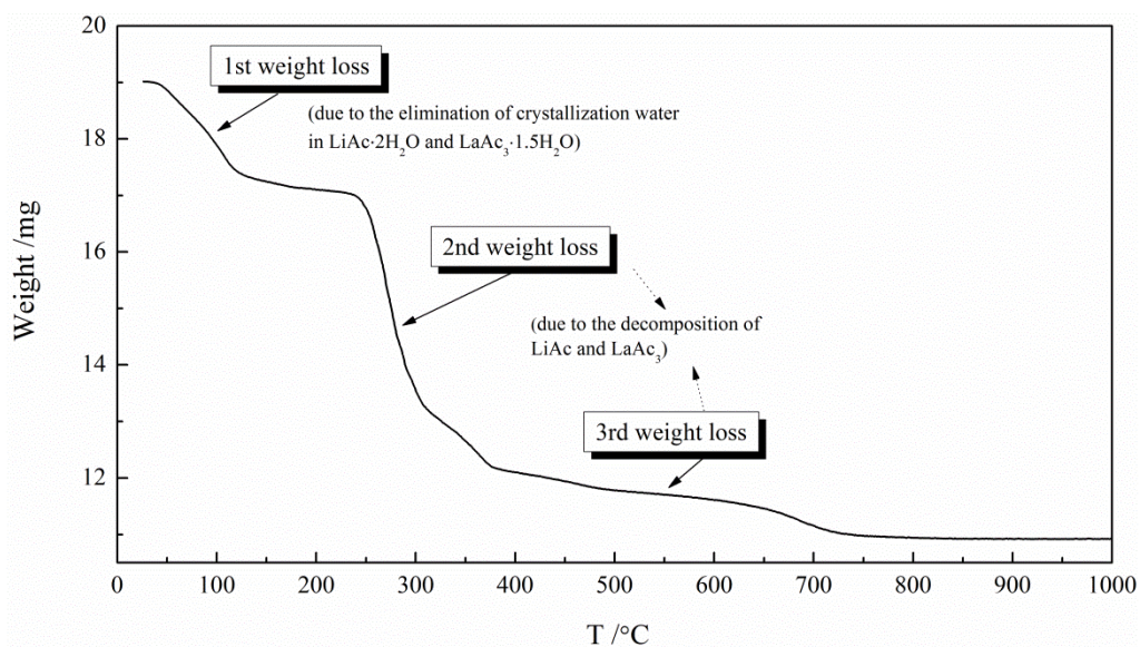
Fig. S1 TGA plot of the precursor powder that contains \text{LiAc}\cdot 2\text{H}_2\text{O} , \text{LaAc}_3\cdot 1.5\text{H}_2\text{O} , and \text{TiO}_2 used for the synthesis of lithium lanthanum titanate.
