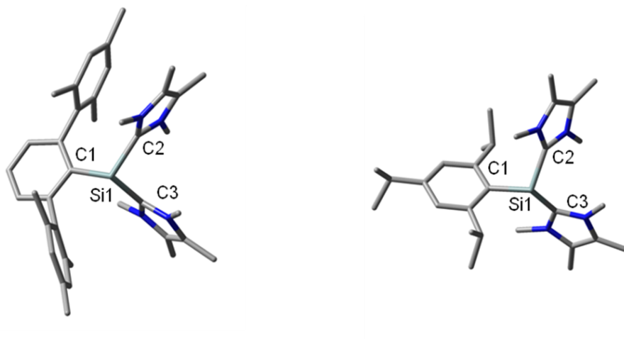
Figure S18. Optimized structure of compounds 1a (left) and 1b (right).
