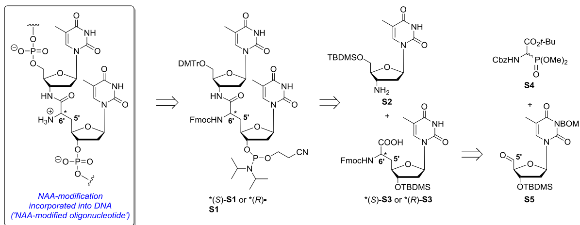
Scheme S1. Retrosynthetic analysis of NAA-modified oligonucleotides.
