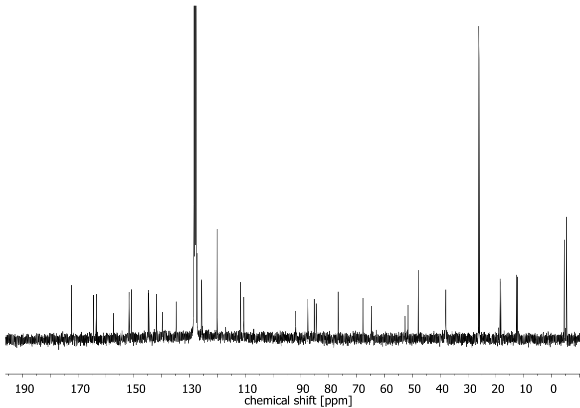
^{13}\text{C} NMR spectrum of ( R )- S9 (75 MHz, \text{C}_6\text{D}_6 , 70 °C)
