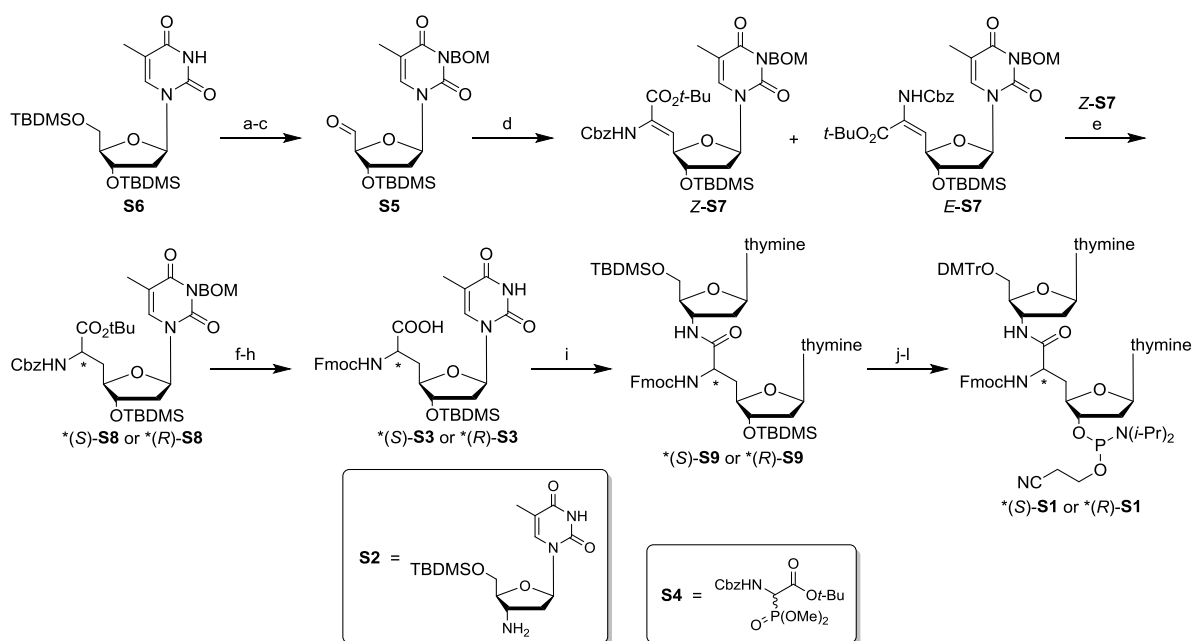
Scheme S2. Synthesis of phosphoramidite building blocks S1 for the preparation of NAA-modified oligonucleotides. Reagents and conditions. (a) BOMCl, NaH, DMF, -10 °C to 0 °C, 3 h, 96%; (b) AcCl, MeOH, -10 °C to 0 °C, 3 h, 59%; (c) IBX, MeCN, reflux, 45 min, 99%; (d) S4 , KO t -Bu, THF, -78 °C to rt, 16 h, 71% Z-S7 , 3% E-S7 ; (e) H 2 (1 bar), cat. , MeOH, rt, 2-7 d, 94% ( S )- S8 (with cat. = ( S,S )-Me-DuPHOS-Rh, d.r. > 98:2), 99% ( R )- S8 (with cat. = ( R,R )-Me-DuPHOS-Rh, d.r. > 98:2); (f) H 2 (1 bar), 10% Pd/C, n -BuNH 2 , MeOH, rt, 24 h, 93% ( S )-isomer, 92% ( R )-isomer; (g) FmocCl, NEt 3 , THF, 0 °C, 30 min, 97% ( S )-isomer, 95% ( R )-isomer; (h) SiO 2 , toluene, reflux, 20 h, 94% ( S )- S3 , 90% ( R )- S3 ; (i) S2 , EDC, HOBt, CH 2 Cl 2 , rt, 16 h, 79% ( S )- S9 , 78% ( R )- S9 ; (j) AcCl, MeOH, 0 °C to rt, 24 h, 92% ( S )-isomer, 91% ( R )-isomer; (k) DMTrCl, pyridine, rt, 16 h, 75% ( S )-isomer, 75% ( R )-isomer; (l) 2-cyanoethyl N,N,N',N' -tetraisopropyl phosphordiamidite, 4,5-dicyanoimidazole, CH 2 Cl 2 , rt, 1 h, 76% ( S )- S1 , 74% ( R )- S1 . From intermediates ( S )- S8 and ( R )- S8 onwards, all reactions were carried out with diastereomerically pure compounds (with either (6' S )- or (6' R )-configuration) and are just summarised in one scheme in the interest of conciseness.
