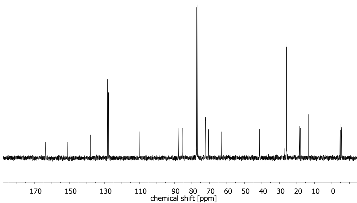
13 C NMR spectrum of S10 (75 MHz, CDCl 3 )
