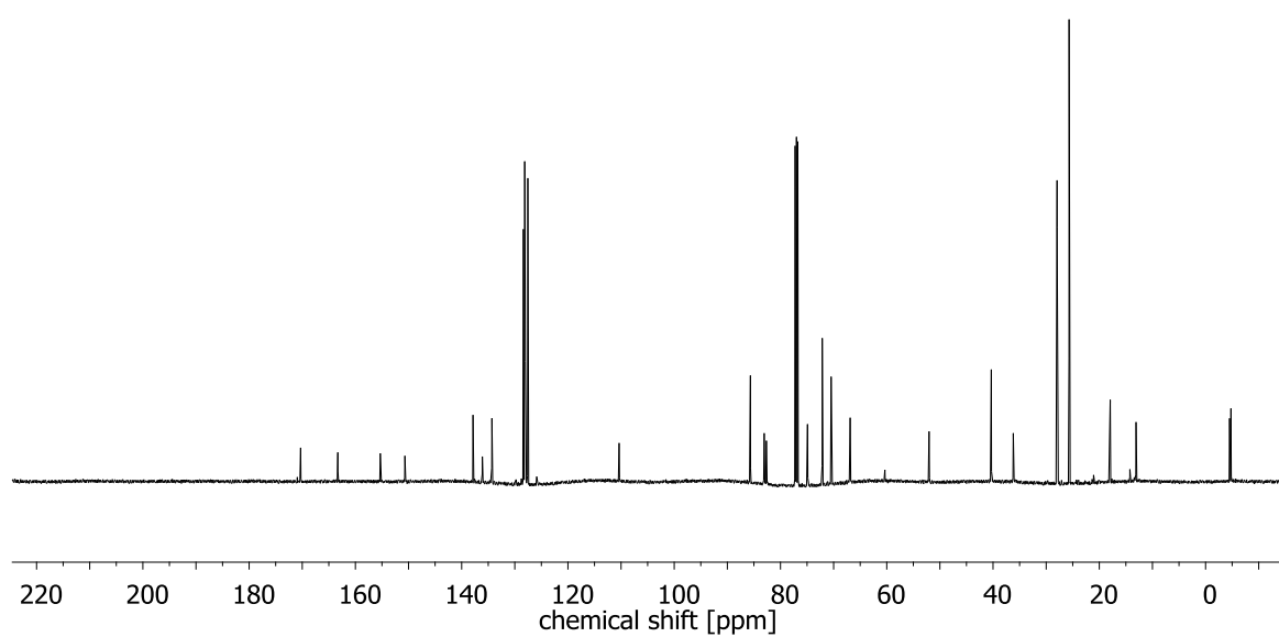
^{13}\text{C} NMR spectrum of ( S )- S8 (75 MHz, \text{CDCl}_3 )
