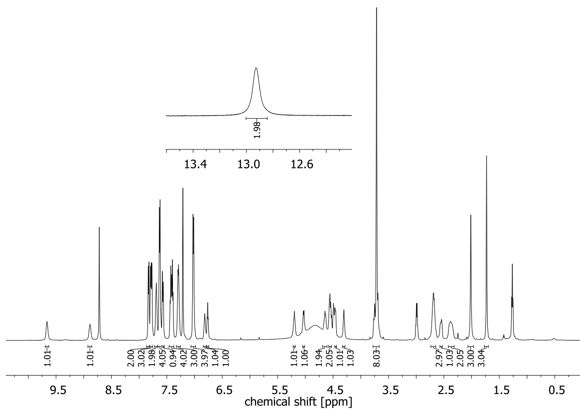
^1\text{H} NMR spectrum of ( S )- S15 (600 MHz, pyridine- d_5 , 50 °C)
