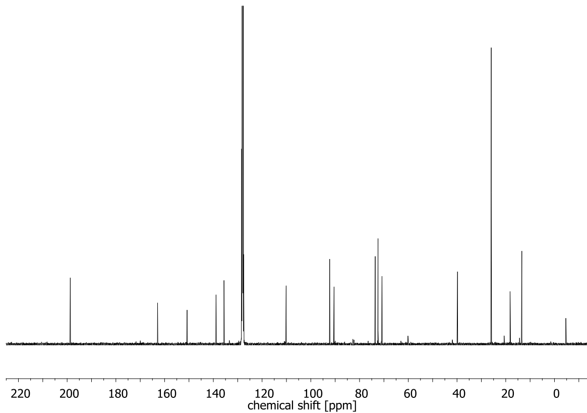
^{13}\text{C} NMR spectrum of S5 (75 MHz, \text{C}_6\text{D}_6 )
