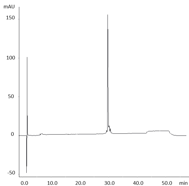
HPLC chromatogram of 7d (5'-GTTGACGTTGACGTTGACGT x TG-3', x = (6'R)-NAA)
