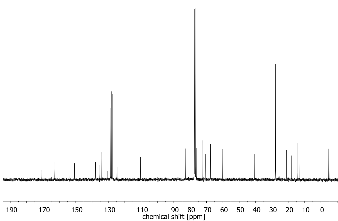
^{13}\text{C} NMR spectrum of Z-S7 (75 MHz, \text{CDCl}_3 )
