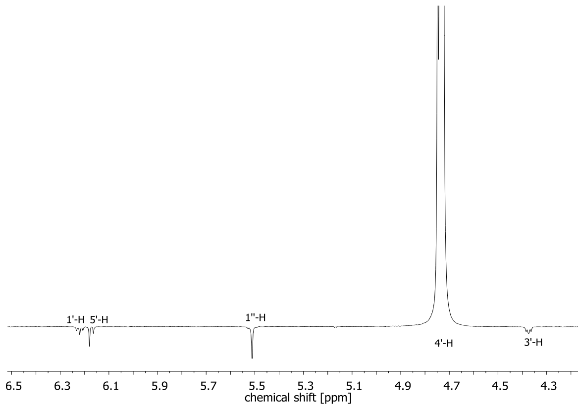
^1\text{H} NOE NMR spectrum of Z-S7 (300 MHz, \text{CDCl}_3 )
