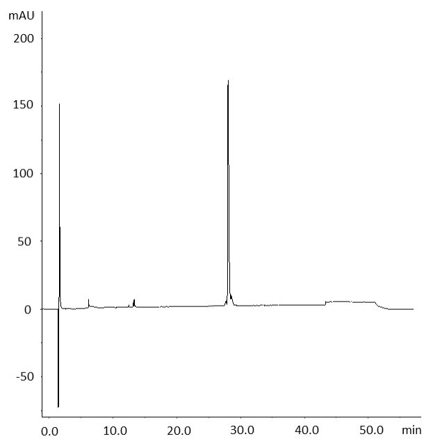
HPLC chromatogram of 6a (5'-GGCACGGT x TTTTTTTGGCACGG-3', x = (6 R )-NAA)
