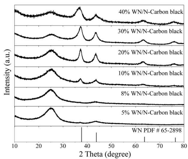
Figure S1. XRD patterns of WN/N-Carbon black with different contents of WN as indicated.
