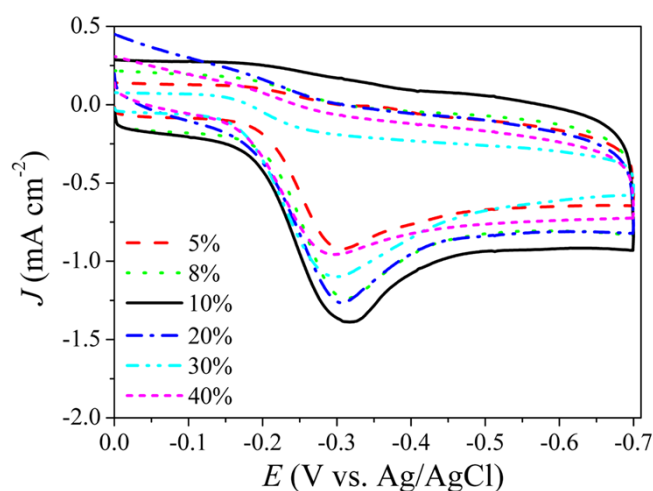
Figure S4. Cyclic voltammograms of WN/N-Carbon black with different contents of WN as indicated in \text{O}_2 -saturated 0.1 M KOH solutions. Scan rate: 50 \text{ mV s}^{-1} .
