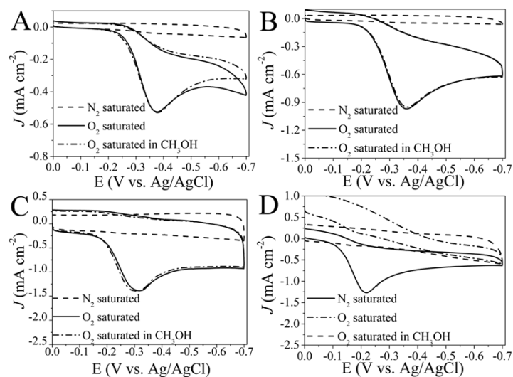
Figure S6. Cyclic voltammograms of A) WN, B) N-Carbon black, C) WN/N-Carbon black and D) Pt/C in N 2 - and O 2 -saturated 0.1 M KOH solutions as well as O 2 -saturated 0.1 M KOH solution with 3 M methanol. Scan rate: 50 mV s -1 .
