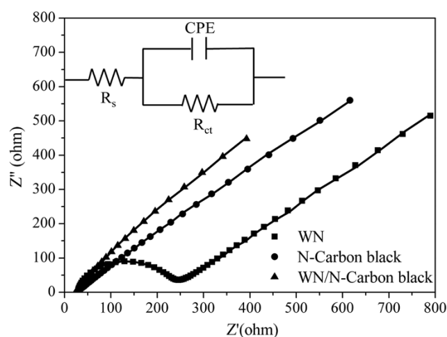
Figure S3. Electrochemical Impedance Spectra of WN, N-Carbon black and WN/N-Carbon black in 5 mM \text{Fe}(\text{CN})_6^{3-/4-} containing 0.5 M KCl from 0.1 Hz to 100 kHz with a signal amplitude of 10 mV. Inset is the equivalent circuit used to fit the impedance spectra. In the equivalent circuit, R_s , R_{ct} , and CPE were the electrolyte resistance, the electron-transfer resistance, and the chemical capacitance.
