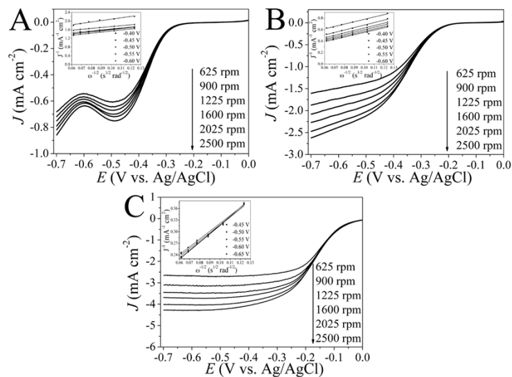
Figure S5. RDE voltammograms at different rotation rates of A) WN, B) N-Carbon and C) Pt/C in O 2 -saturated 0.1 M KOH solutions. Sweep rate: 5 mV s -1 . Insets are the corresponding K-L plots at different potentials.
