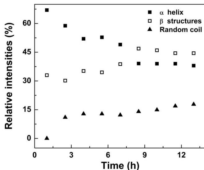
Figure S4. Effects of 70 nm AuNPs on the relative amount of \alpha -helix structure (■), \beta -structure ( \beta -sheet and \beta -turn, □), and random coil (▲).
