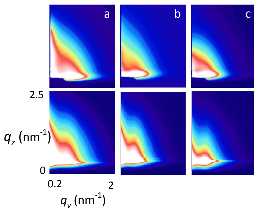
Fig. S5 GISAXS data (first row) and simulated GISAXS patterns (second row) of the IGZO film annealed at 300°C (a), 380°C (b), and 450°C (c).
