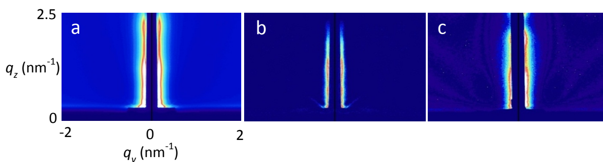
Fig. S3 X-ray scattering data of the IGZO film annealed at 200^\circ\text{C} . GISAXS data (a), AGISAXS data in the vicinity of the K-edge of Zn (b), and AGISAXS data in the vicinity of the K-edge of Ga (c).
