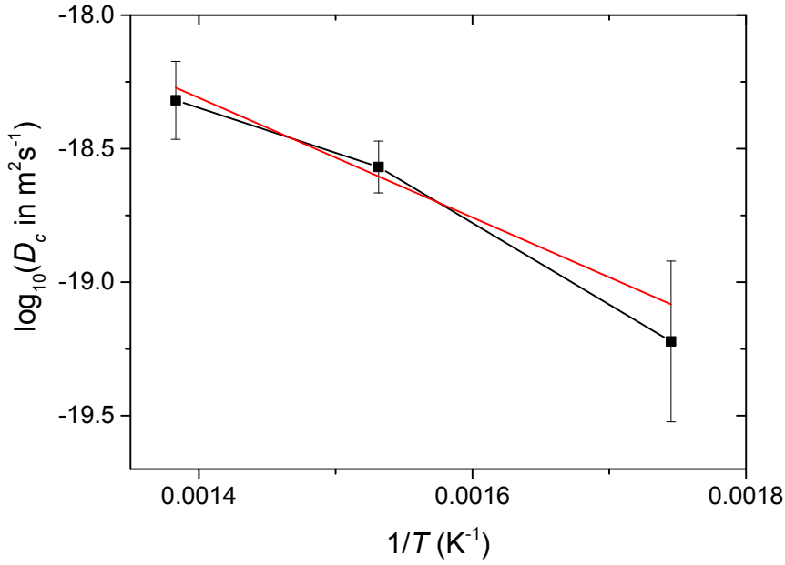
Fig. S6 Arrhenius diagram of Ga diffusion coefficient. The black curve corresponds to the estimated diffusion constants from the AGISAXS data. The red line corresponds to the linear fit.
