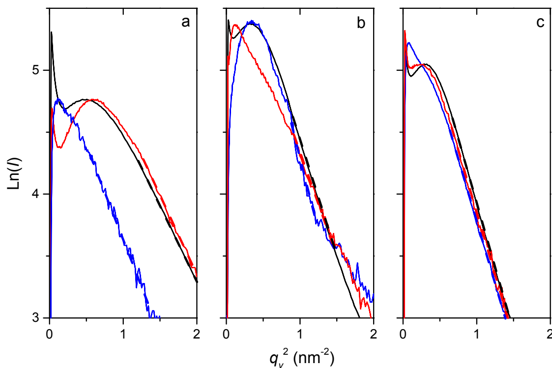
Fig. S4 \text{Ln}(I) as a function of q_y^2 for the linescans of the fourth row in Fig. 3 for IGZO films annealed at 300^\circ\text{C} (a), 380^\circ\text{C} (b), and 450^\circ\text{C} (c). The dash line corresponds to the linear fit.
