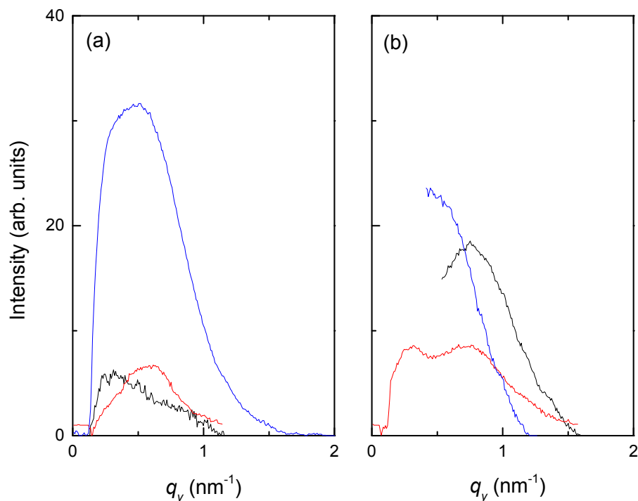
Fig. S7 GISAXS q_y linescans at q_z = 0.5 \text{ nm}^{-1} from the Zn-rich nanoclusters (a) and from the Ga-rich nanoclusters (b) for films annealed at 300°C (black line), 380°C (red line), and 450°C (blue line).
