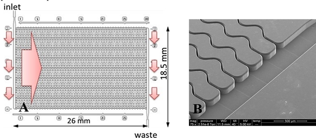
Figure S1. (A) AutoCAD drawing of the z-configuration cell selection device, which in this format contains 50 high aspect ratio parallel, sinusoidal channels with dimensions of 25 \times 150 \mu\text{m} (w x h). The large arrow indicates the sample flow direction through the microchannels. (B) SEM image of the cell selection bed showing the input channel and the associated sinusoidal channels. The sinusoidal channels contained the mAbs, which were covalently anchored to the polymer surface via an amide bond formed between the polymer's surface confined carboxylic acid groups and a primary amine group resident within the mAb primary structure (direct attachment) or to a 5' primary amine group resident on the ssDNA linker that contained a uracil residue for clipping via USER™ (see Scheme S1).
