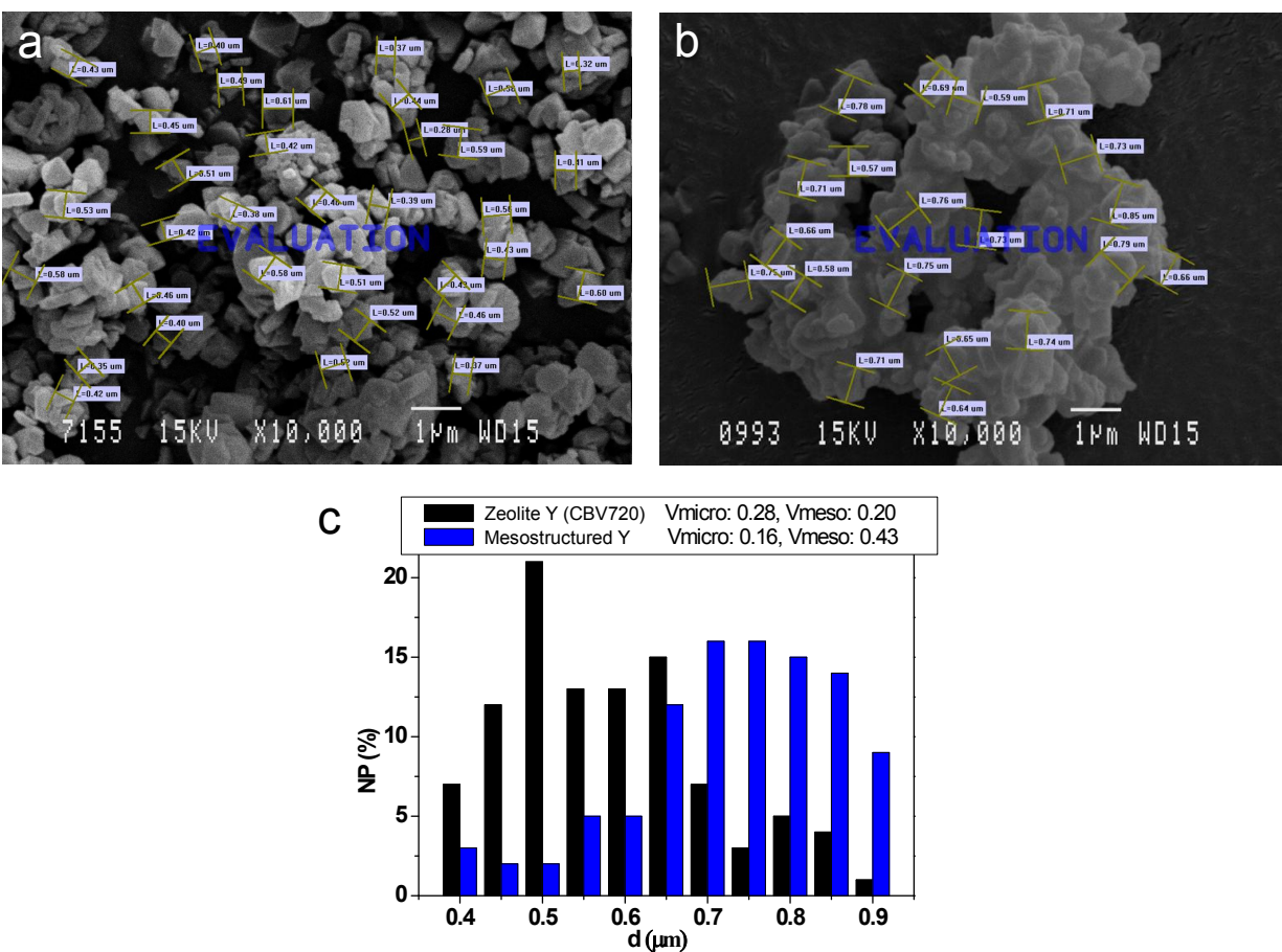
Fig. S1 SEM micrographs of a) the starting zeolite Y (CBV720), b) mesostructured Y zeolite, and c) their histograms indicating the size distribution in the SEM images.
