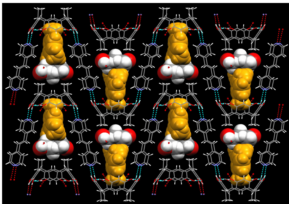
Fig. S2 1D wave-like structure of 9.
