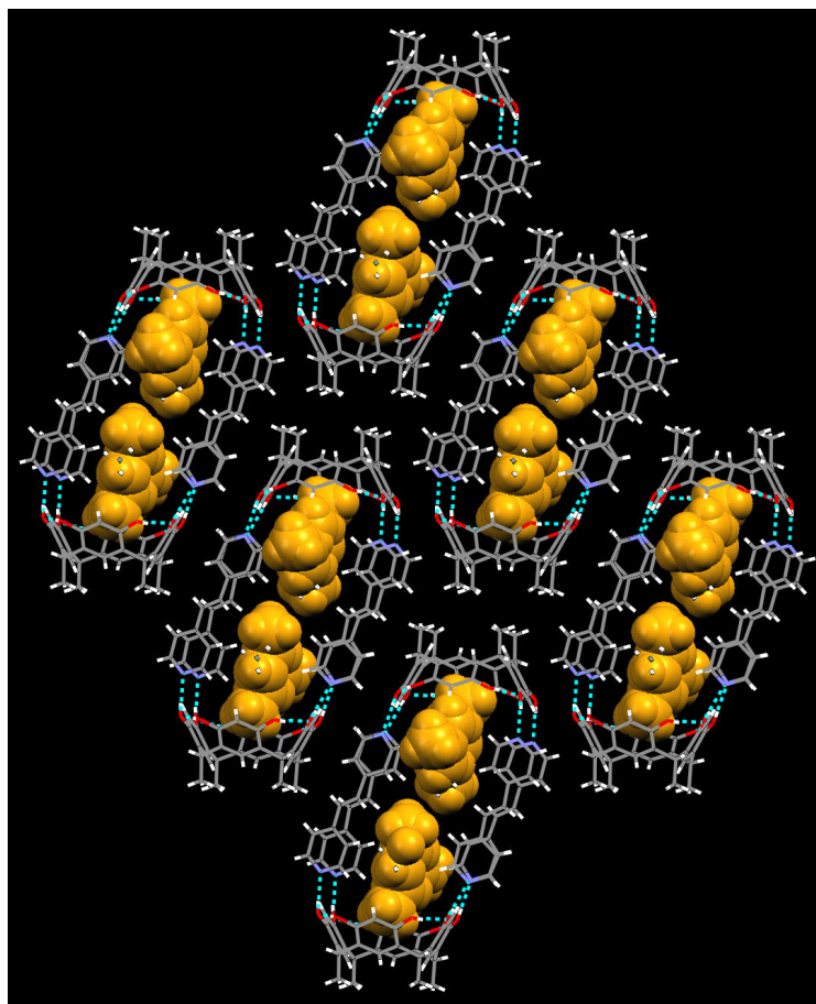
Fig. S3 Carcerand structure of 10.
