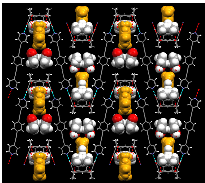
Fig. S4 1D wave-like structure of 12.
